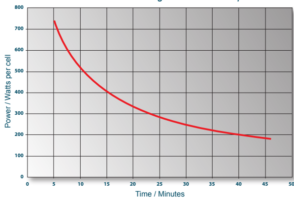
NSB12-400 Discharge Curve to 1.67 vpc
